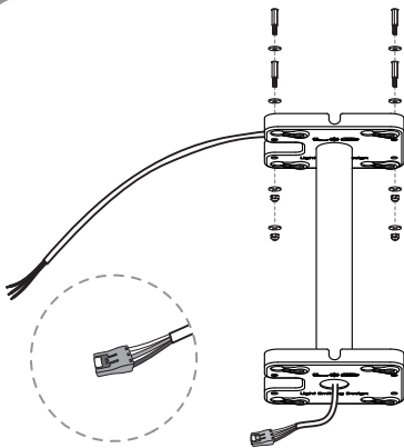
Quick Connect
